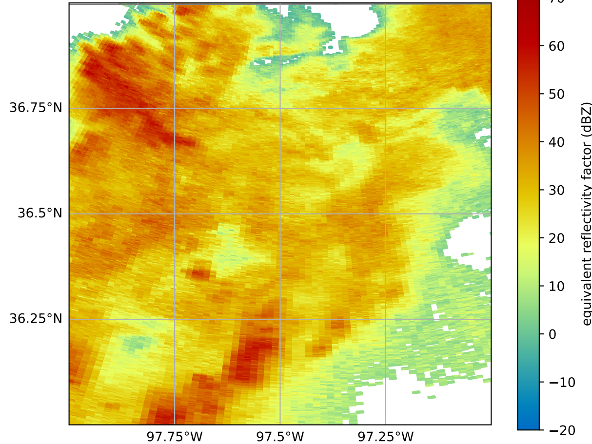
KICT 0.9 Deg. 2011-05-20T08:15:24Z Equivalent reflectivity factor
