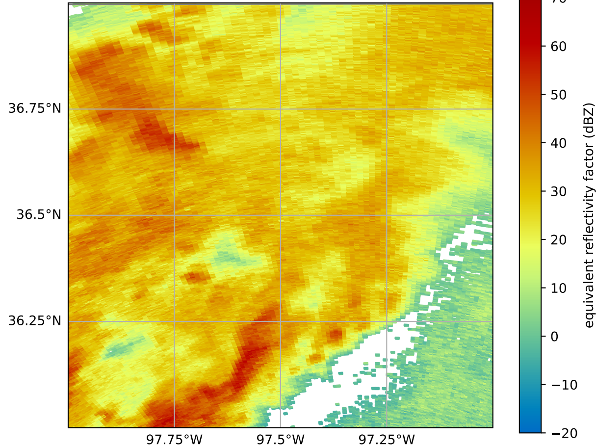
KTLX 0.9 Deg. 2011-05-20T08:15:03Z Equivalent reflectivity factor
