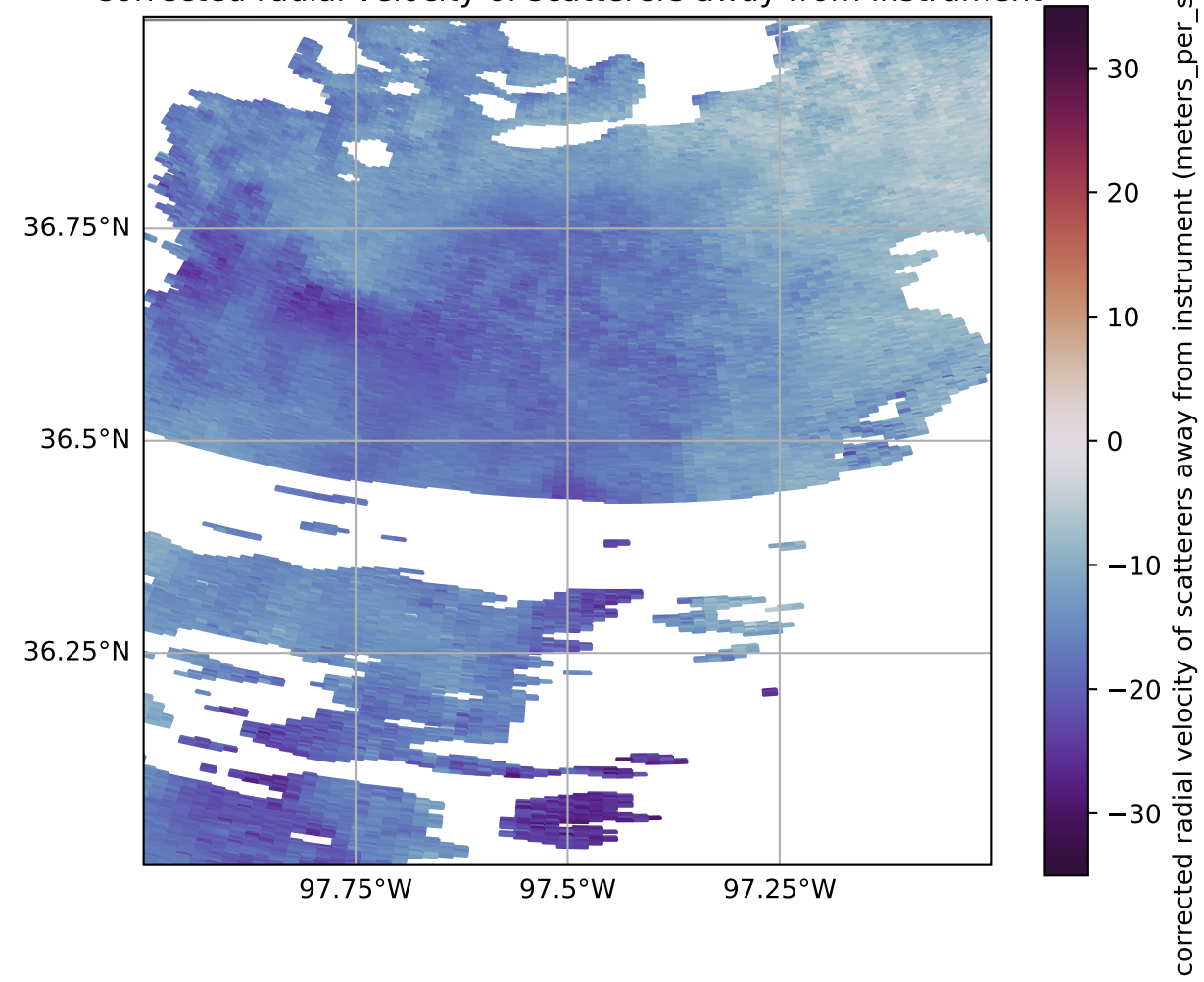
KICT 0.9 Deg. 2011-05-20T08:15:24Z Corrected radial velocity of scatterers away from instrument
