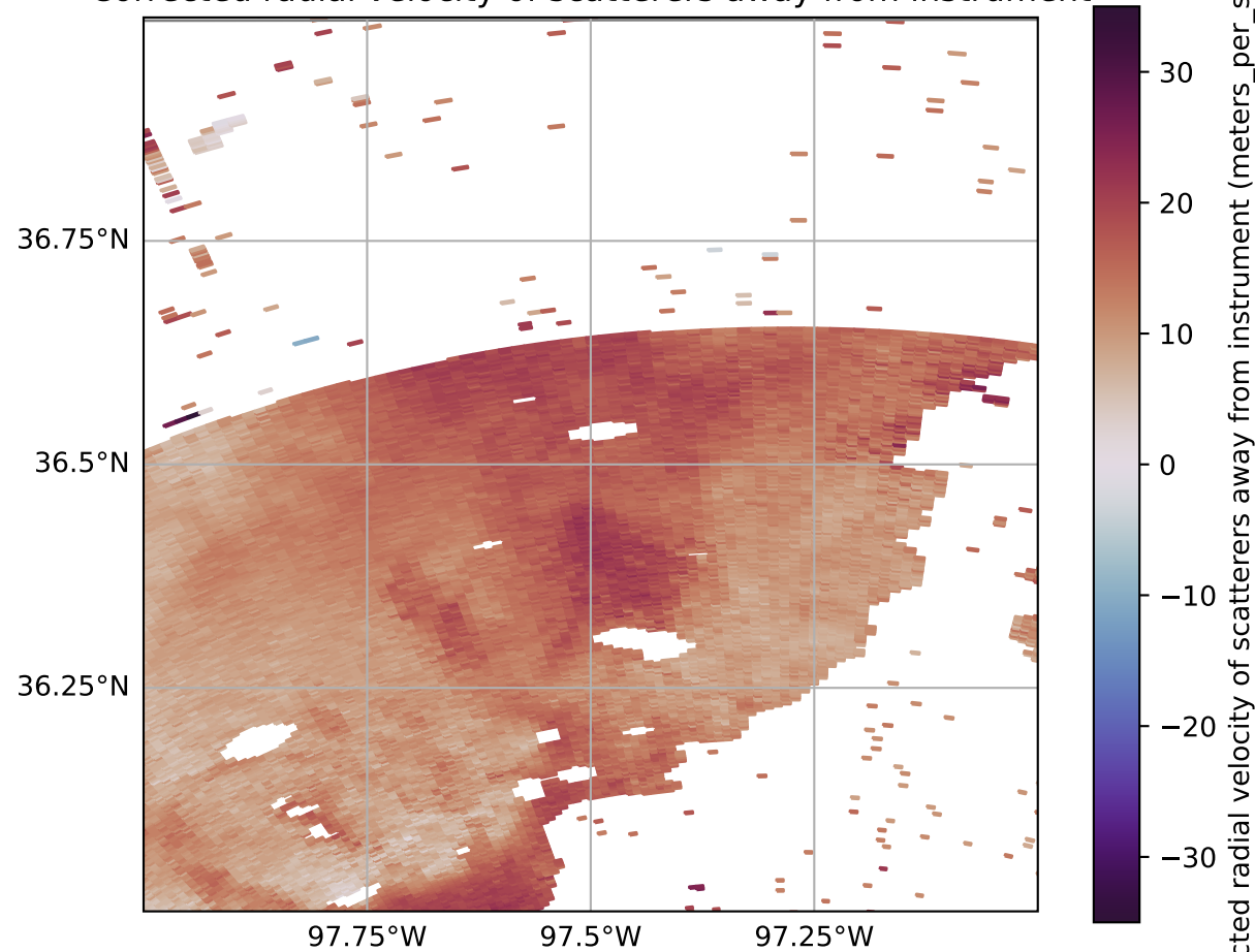
KTLX 0.9 Deg. 2011-05-20T08:15:03Z Corrected radial velocity of scatterers away from instrument
