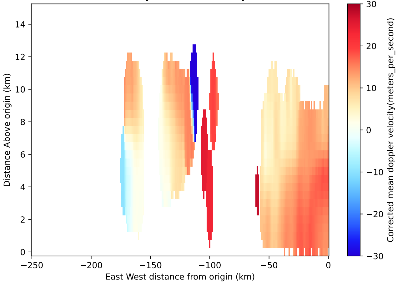
KICT 128.0 km south of origin 2011-05-20T08:14:44Z Corrected radial velocity of scatterers away from instrument
